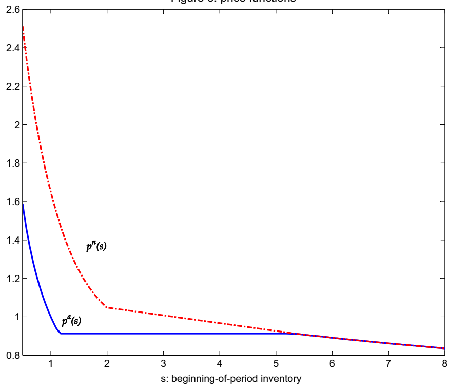
Figure 3: price functions
