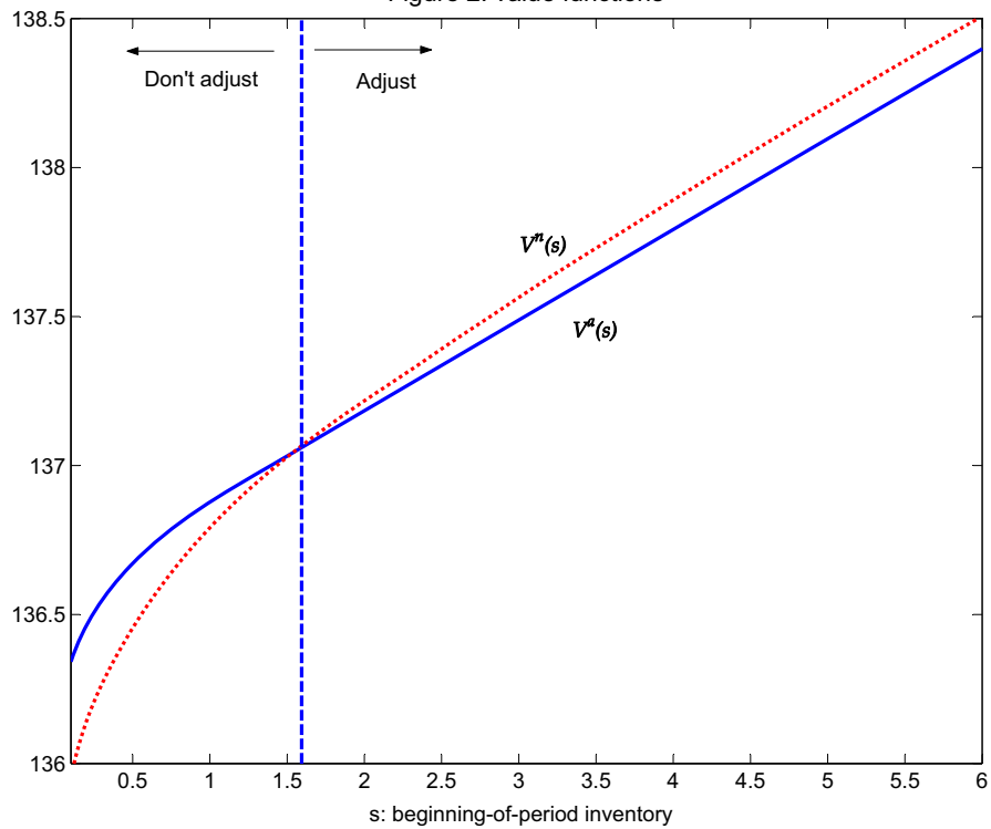
Figure 2: value functions
