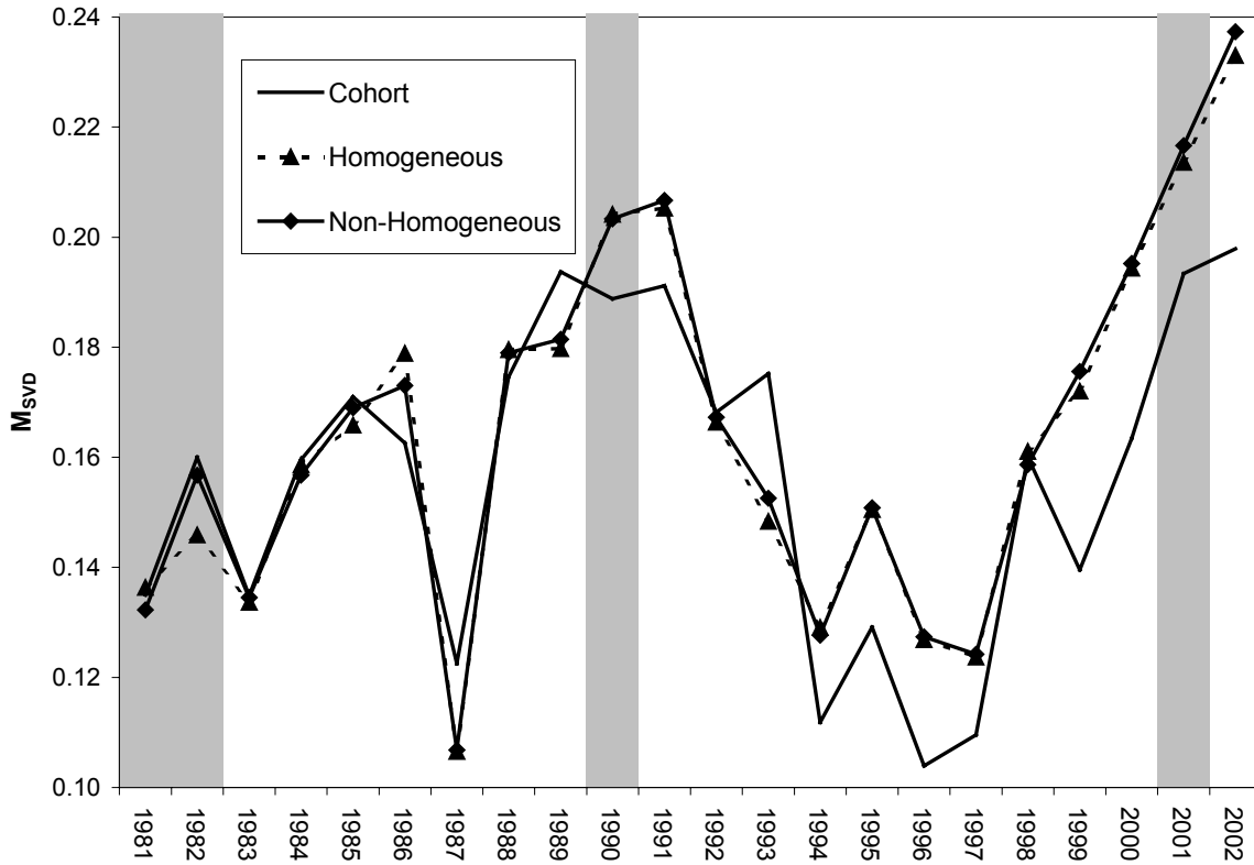
Figure 2: M_{SVD} of annual mobility matrices, comparing three estimation methods: cohort and two duration based methods, parametric (imposing time homogeneity) and nonparametric (relaxing time homogeneity). S&P, U.S., 1981-2002. Shaded areas correspond to NBER recession periods.
