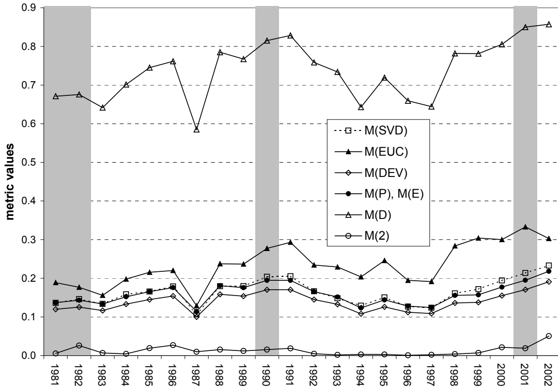
Figure 1: Comparison of Matrix Metrics: S&P, U.S., 1981-2002, using the duration based (time homogeneous) method. Metrics are defined in eq. (2.7) for M_D , M_E , M_P and M_2 , eq. (3.4) for M_{SVD} , and eq. (3.8) for M_{euc} and M_{dev} . Shaded areas correspond to NBER recession periods.
