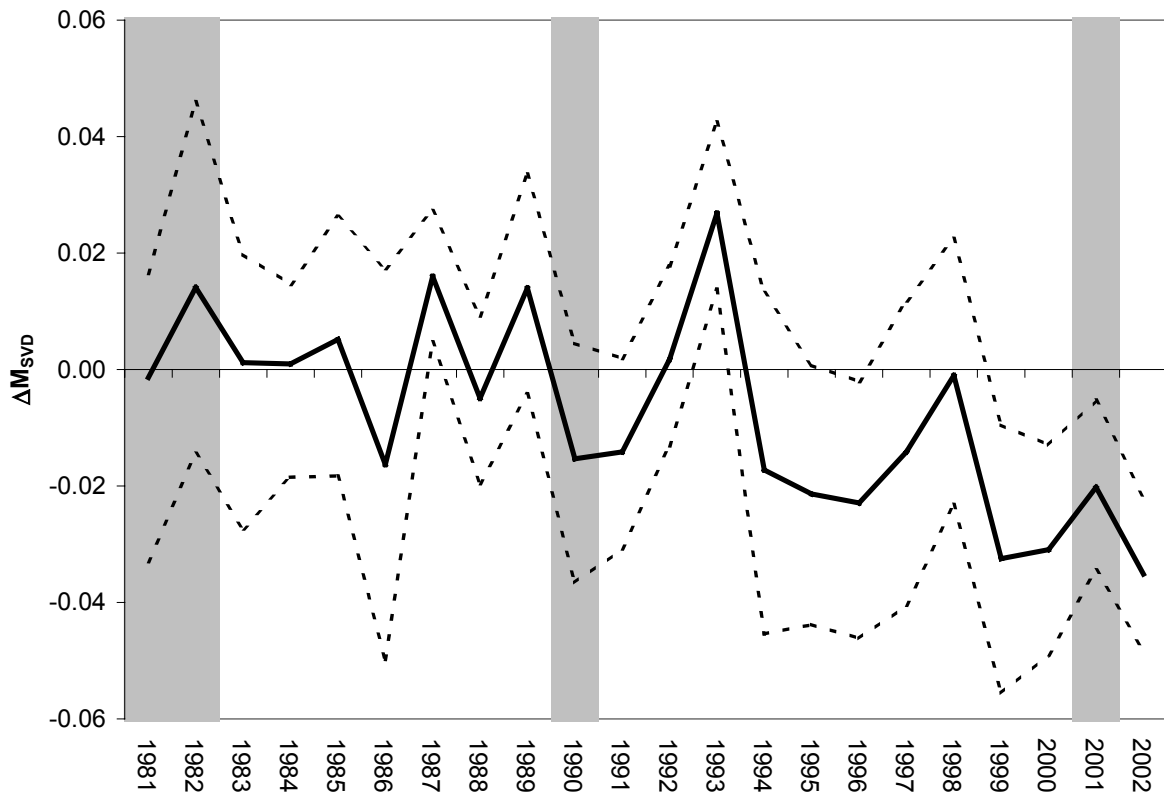
Figure 5: Bootstrapped 95% confidence bands of \Delta M_{SVD}(\hat{\mathbf{P}}_{coh}, \hat{\mathbf{P}}_{hom}) , assessing the difference between cohort and homogeneous duration estimation methods for each yearly migration matrix. S&P, U.S., 1981-2002. Shaded areas correspond to NBER recession periods.
