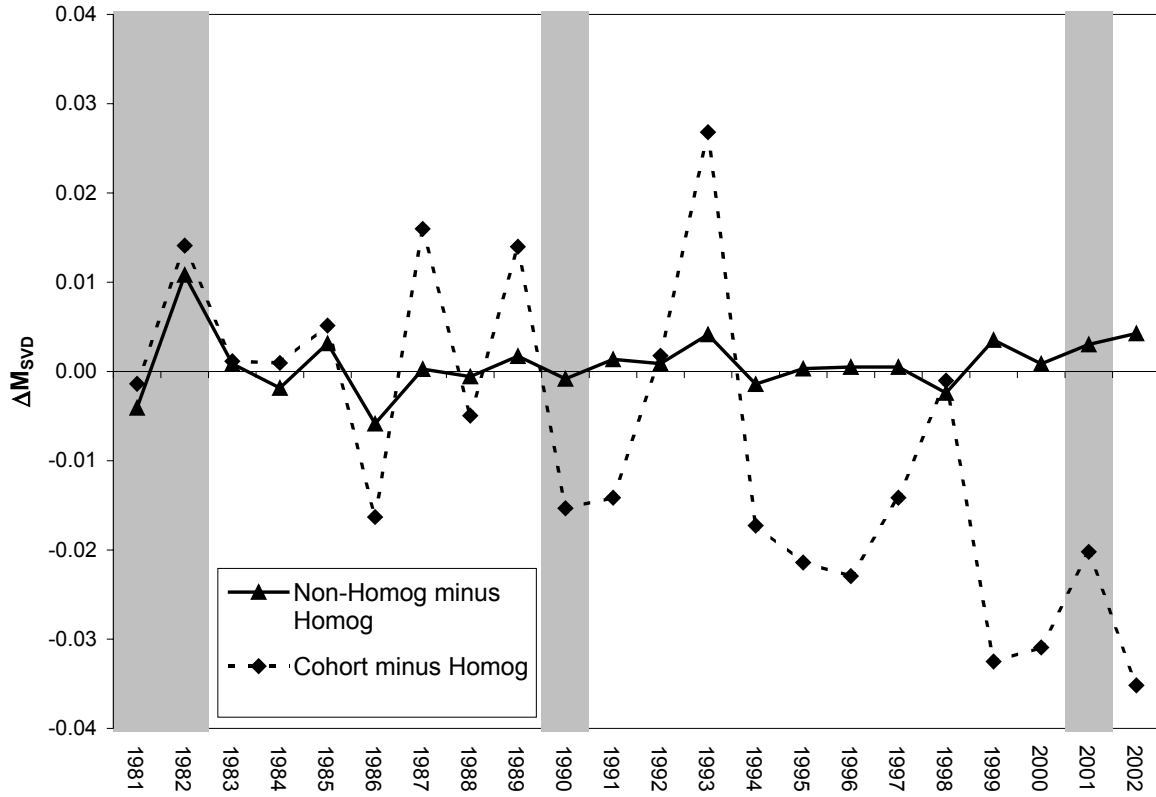
Figure 4: \Delta M_{SVD} assessing differences in migration matrices estimated using different estimation methods, always relative to the time homogeneous (parametric) duration estimator. S&P, U.S., 1981-2002. Shaded areas correspond to NBER recession periods.
