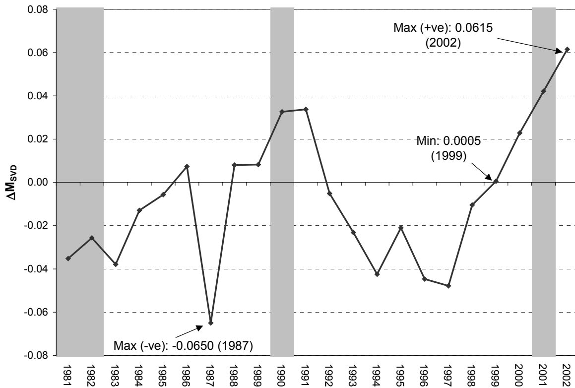
Figure 3 Using differences in M_{SVD} to assess the time-evolution of the deviation of the annual migration matrix from the full-sample (long-run average) estimated matrix, 1981-2002. S&P, U.S., Homogeneous Duration. Shaded areas correspond to NBER recession periods.
